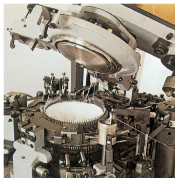
Circular tube knitting machine
